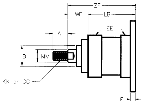
MF2 RECTANGULAR FLANGE (REAR)
