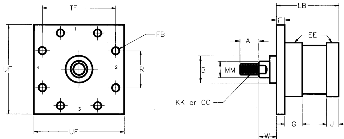
MF5 SQUARE FLANGE (FRONT)
