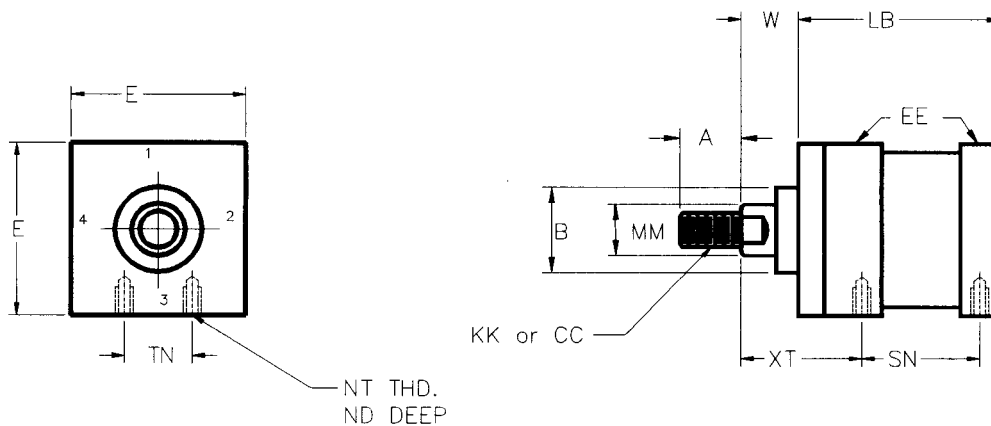
MS4 SIDE TAPPED
