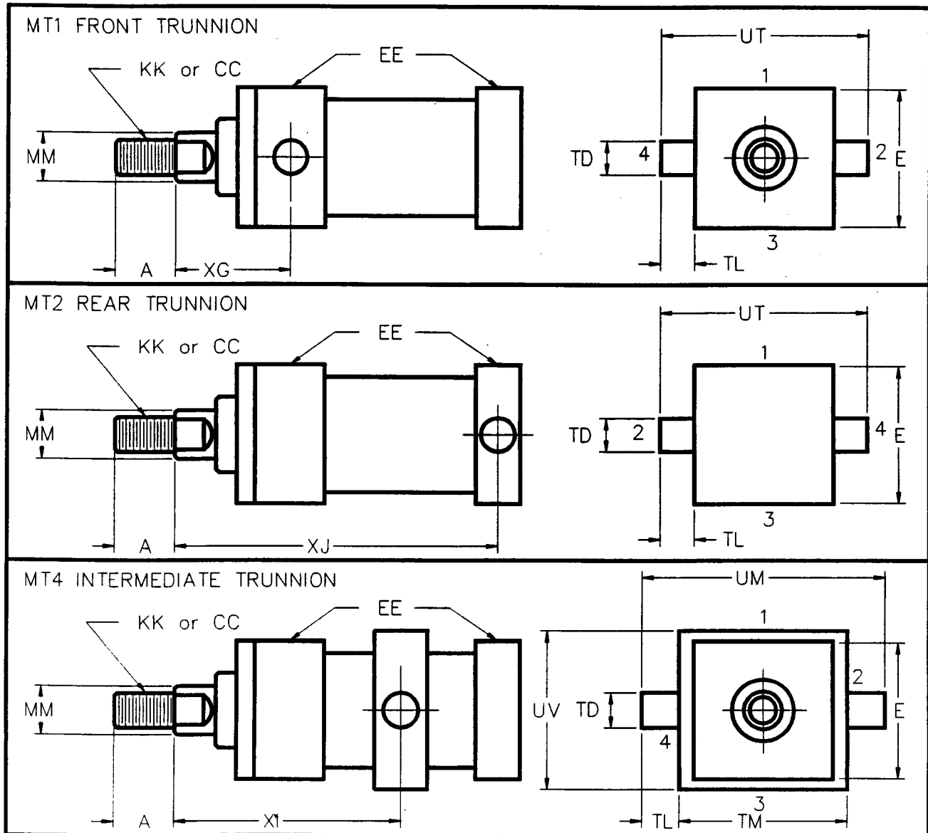
ENVELOPE AND MOUNTING DIMENSIONS
