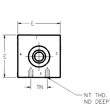
MS4 SIDE TAPPED
